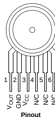
Top view
